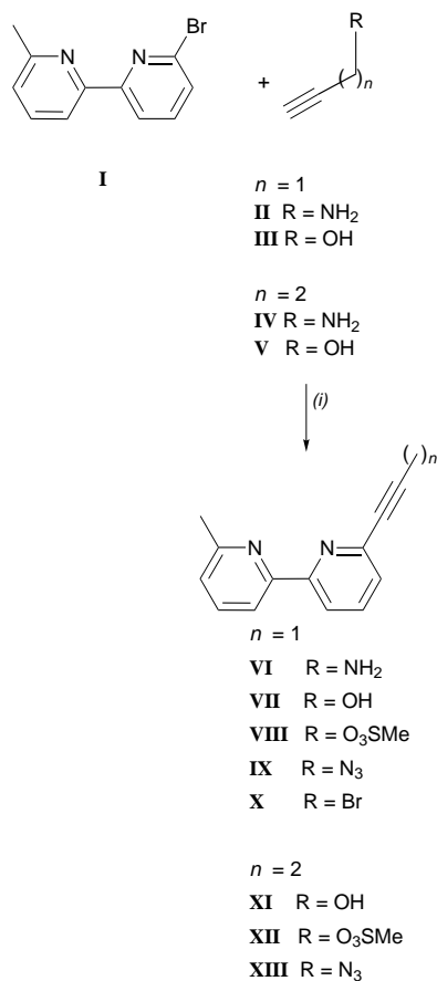
Scheme 2 (i) \text{Pd}^0 , \text{NHPr}^t_2 , \text{Cu}^I , tetrahydrofuran (thf)
