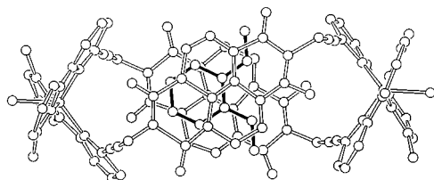
Fig. 4 A ball and stick depiction of complex 2 indicating the disposition of the bound o -dimethoxybenzene (black) with respect to the pyromellitimide spacers
