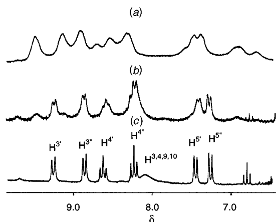
Fig. 5 The 400 MHz ^1\text{H} NMR spectra at 300 K of the copper(I)- \text{L}^1 complex 4 in \text{CD}_3\text{CN} (a) and after the addition of 3 (b) and 24 equivalents m -methoxybenzene (c)
